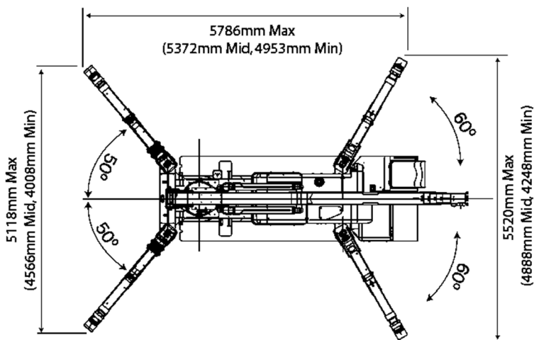
Diagram shows outriggers at maximum position
